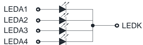
BACKLIGHT CIRCUIT
