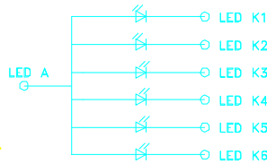
B/L CIRCUIT DIAGRAM If=120mA Vf=3.3V typ
